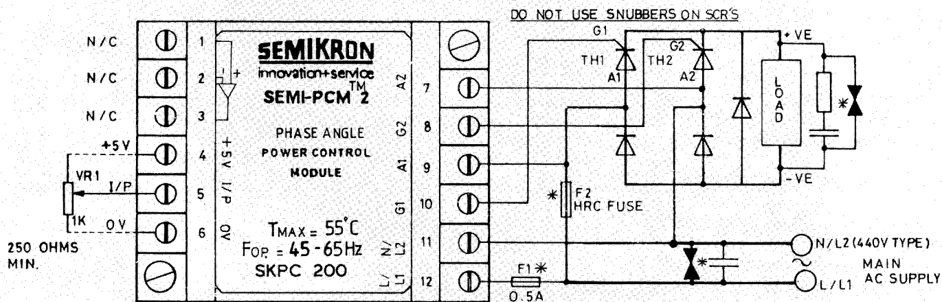
ALTERNATIVE HALF CONTROLLED D.C. BRIDGE (B2HKF)
