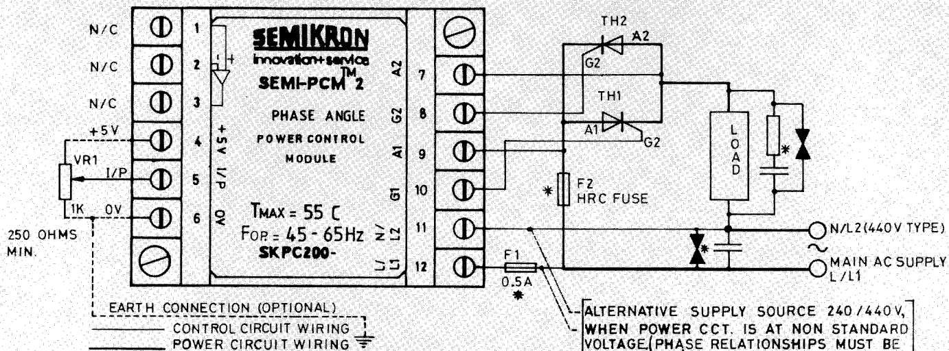
BASIC A.C. REGULATOR (WIC) WIRING
