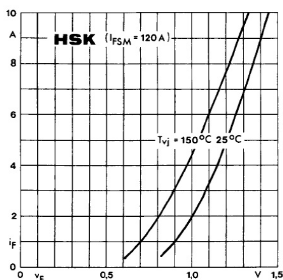
Fig. 5 b Forward characteristic of a single chip
