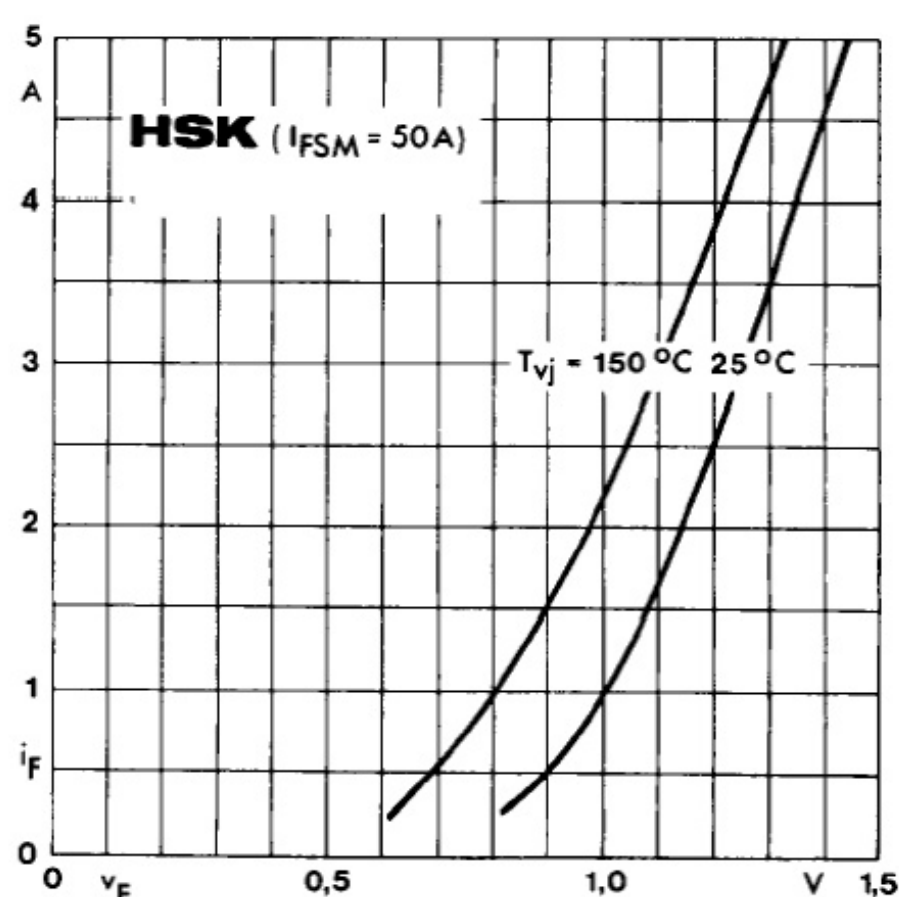
Fig. 5 a Forward characteristic of a single chip
