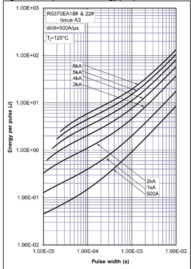
Figure 18 - Square wave energy per pulse
